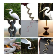
Dataset examples
