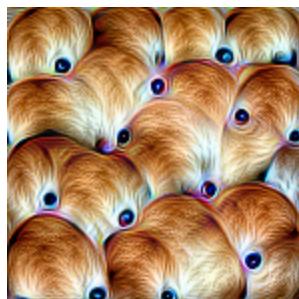
Simple optimization
