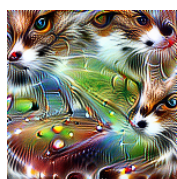
Simple Optimization
