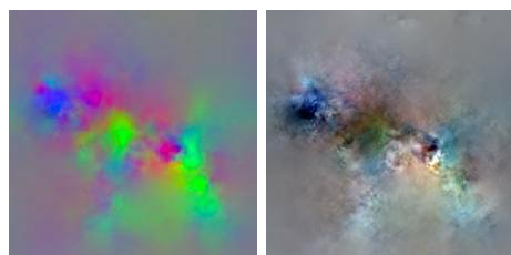
Correlated Colors
