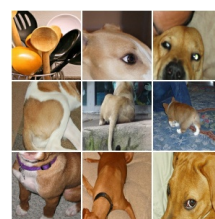
Dataset examples
